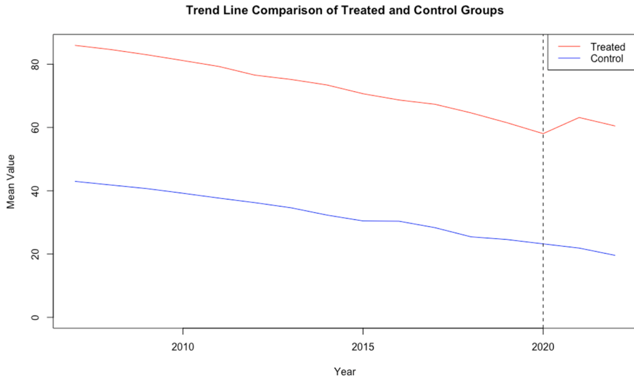
Fig. 2. Parallel Trend.
