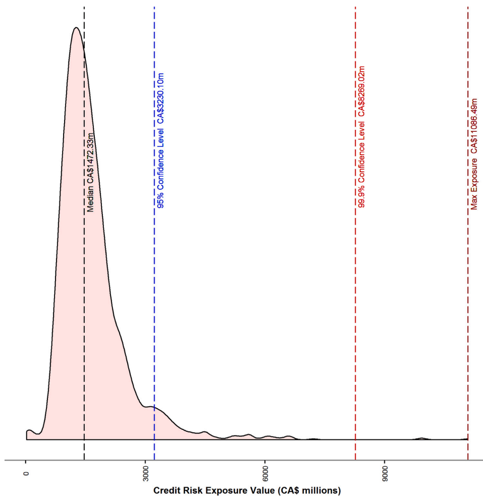
Fig. 3. LVTS simulated multiple default total Maximum Additional Settlement Obligations (Max ASO).
