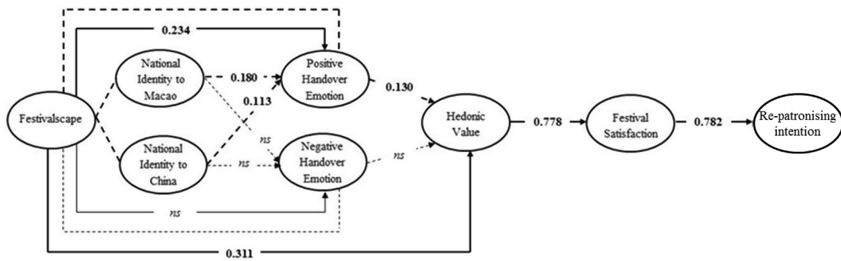
Fig. 3. Model estimation results.
